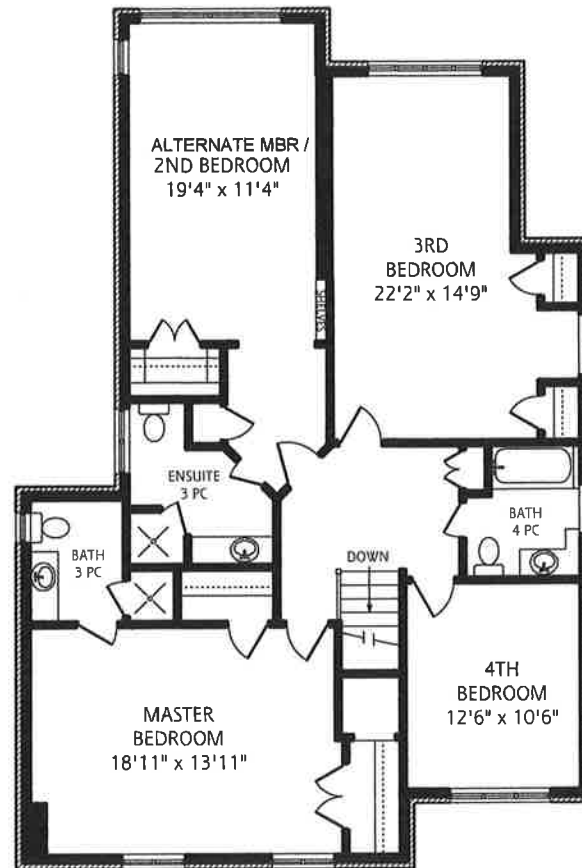
SECOND FLOOR 1,530 SQUARE FEET
