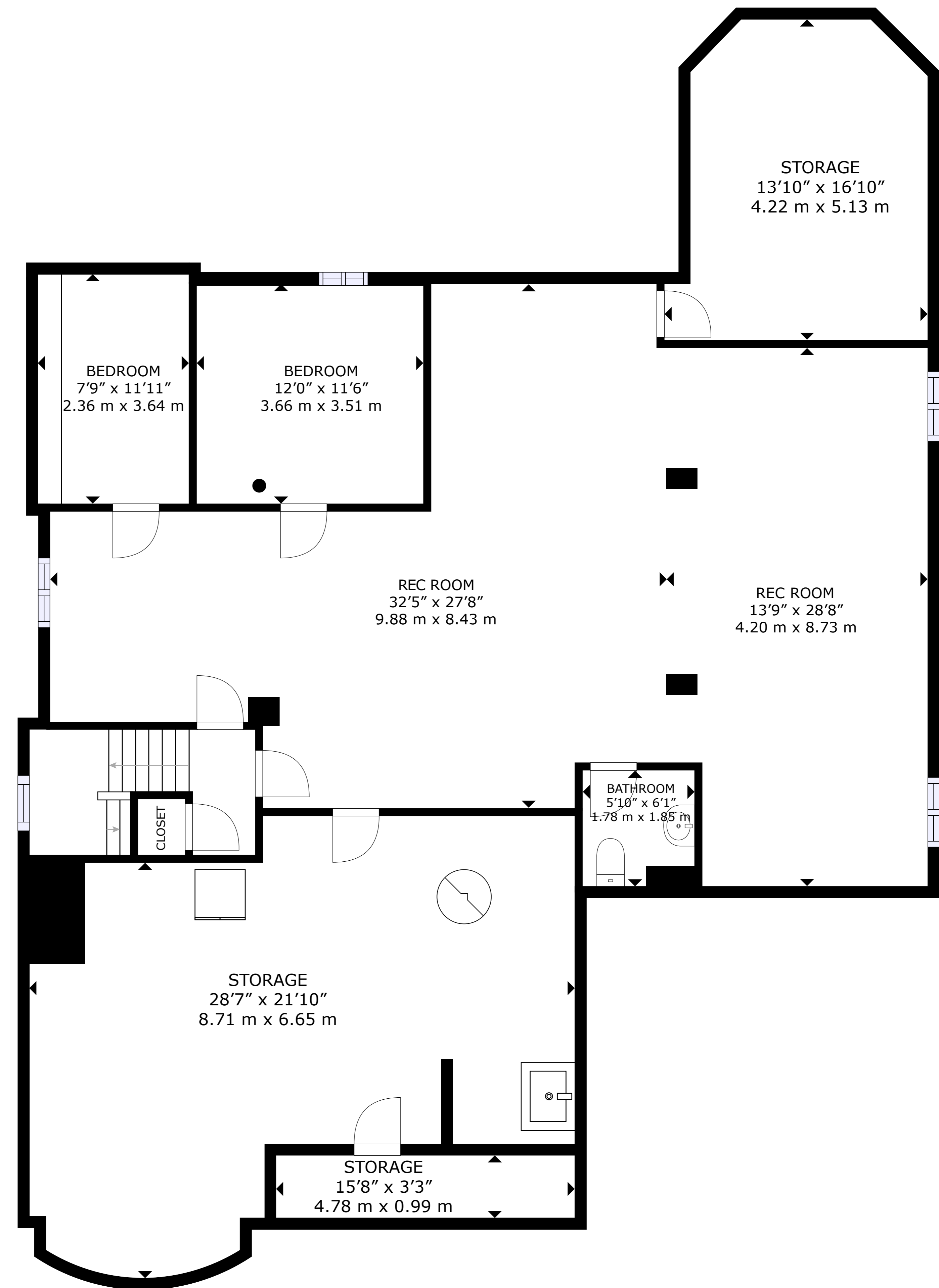
Lower Level
