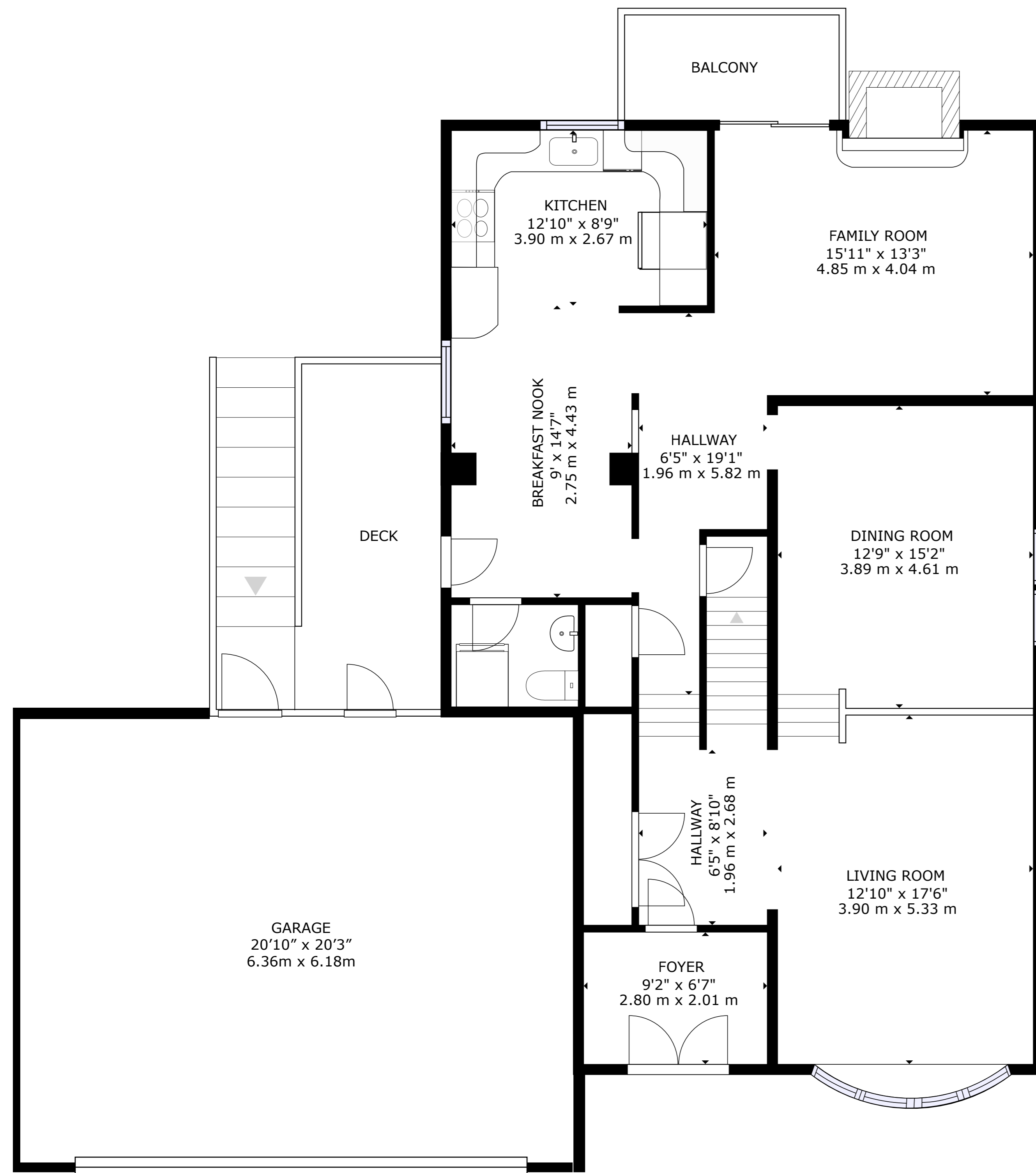
MAIN LEVEL
